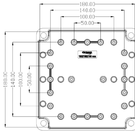
Internal View
