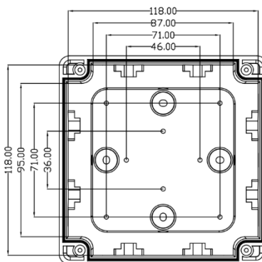
Internal View
