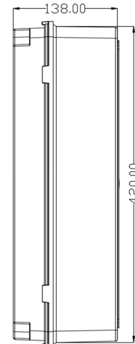
Side View
