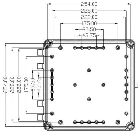
Internal View
