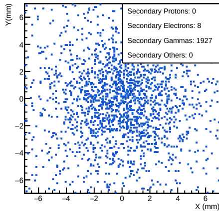
Hits of secondary particles
