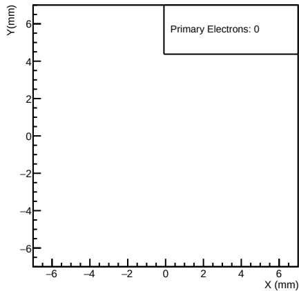
Hits of primary electrons
