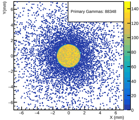
Hits of primary gammas
