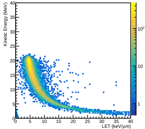
All Particles
