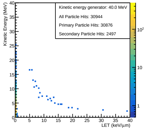
Secondary Particles
