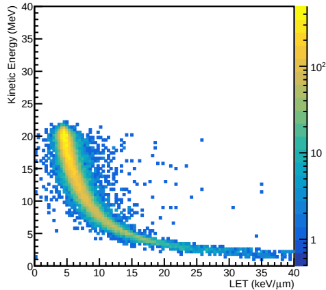
Primary Particles
