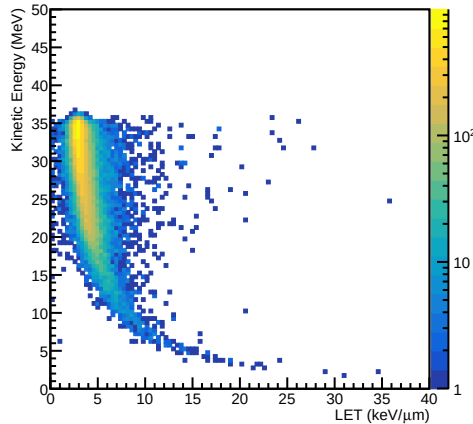
Primary Particles
