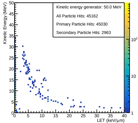
Secondary Particles
