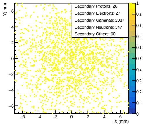
Hits of secondary particles
