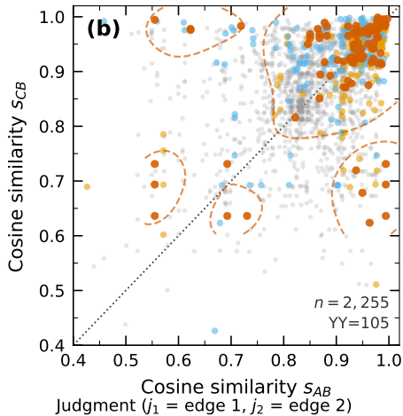
Type 2: A \rightarrow B \leftarrow C
