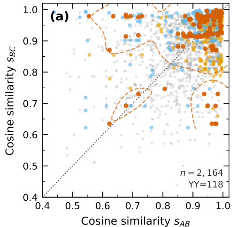
Type 1: A \rightarrow B \rightarrow C
