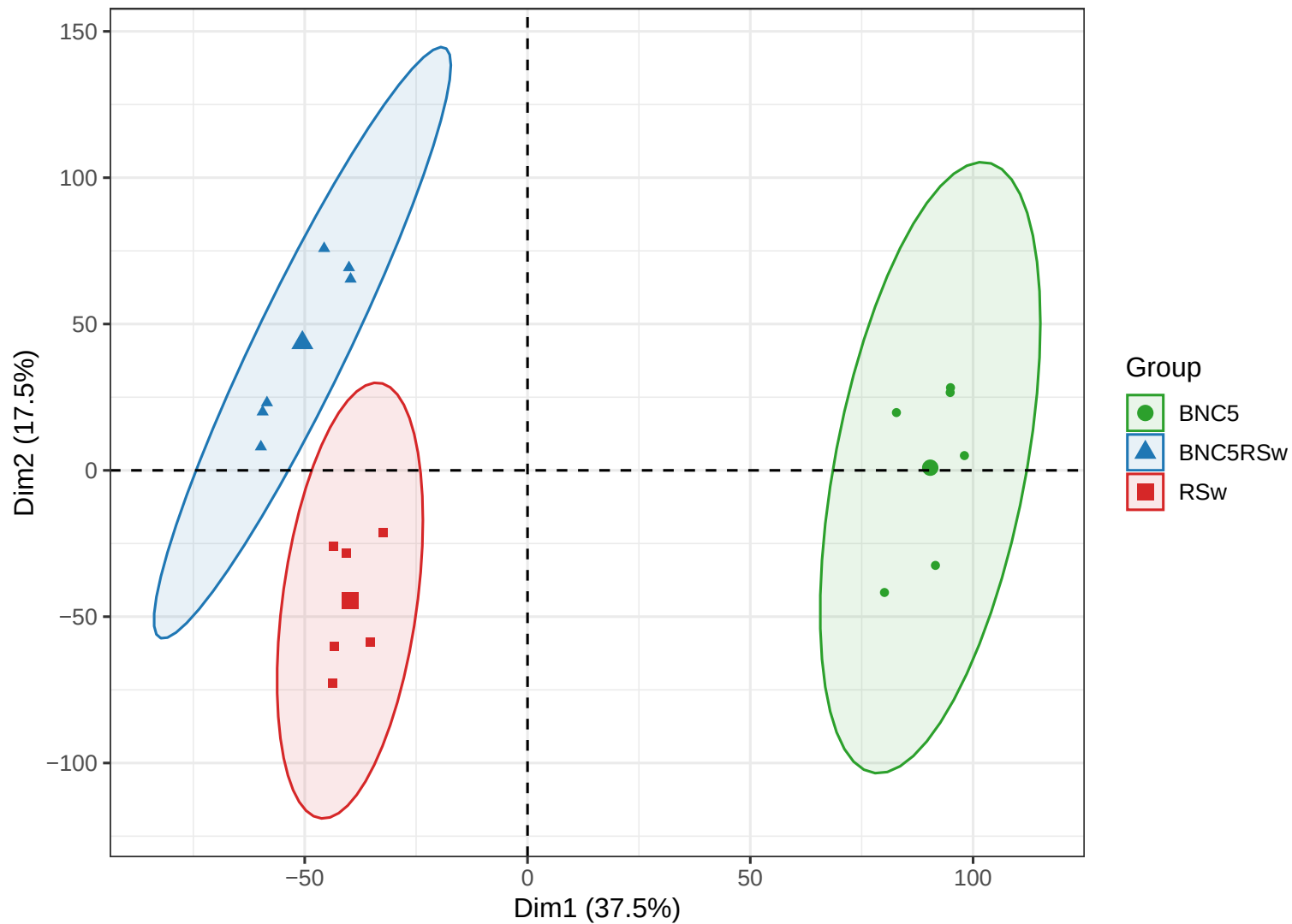
PCA — Biological Groups
