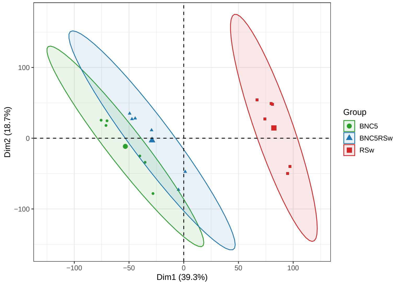
Supernatant PCA — PC1: 39.3%, PC2: 18.7%
