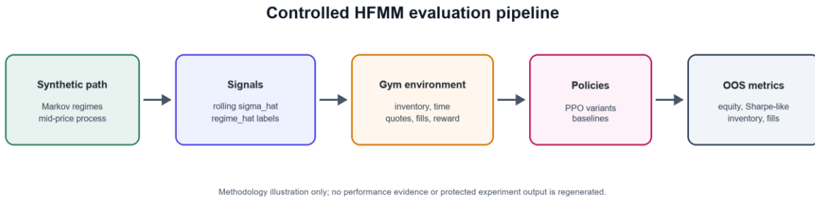
Figure 4.1. Methodology-only HFMM evaluation pipeline. Synthetic market paths produce \sigma_{\hat{}} and \text{regime}_{\hat{}} signals, which feed the Gymnasium environment, PPO variants, baselines, and out-of-sample metrics. Generated by scripts/figures/gen_pipeline_architecture_figure.py ; this illustration is not performance evidence.
