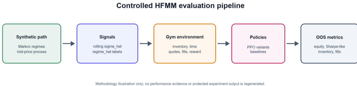
Figure 4.1. Methodology-only HFMM evaluation pipeline. Synthetic market paths produce \sigma_{\hat{}} and regime_hat signals, which feed the Gymnasium environment, PPO variants, baselines, and out-of-sample metrics. Generated by scripts/figures/gen_pipeline_architecture_figure.py; this illustration is not performance evidence.
