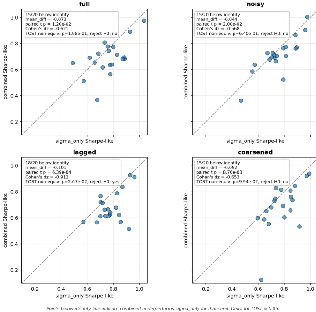
Paired-seed comparison: combined vs sigma_only across conditions
