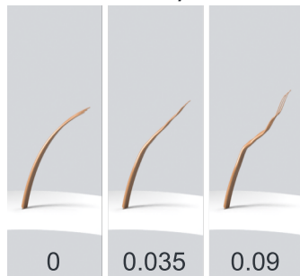
Micro-frizz a/\ell
