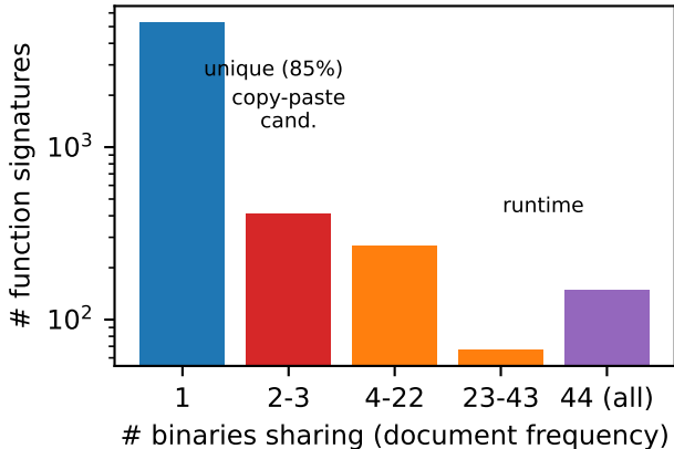
Cross-binary DF spectrum (44 executables)
