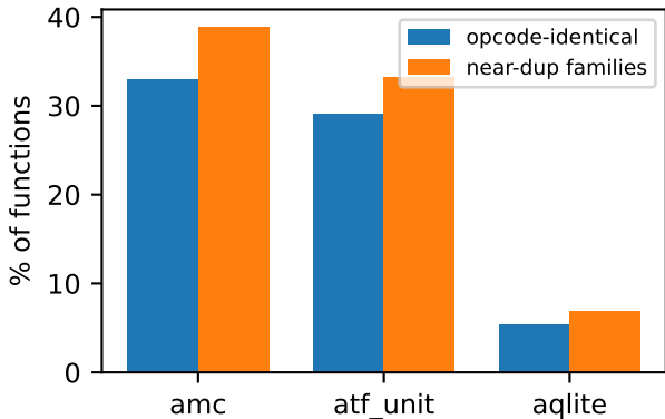
Near-duplicate prevalence
