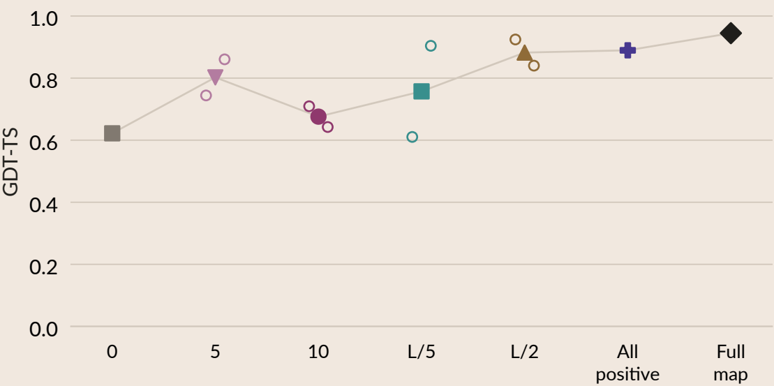
8wrx_A • depth 4 • L = 88
