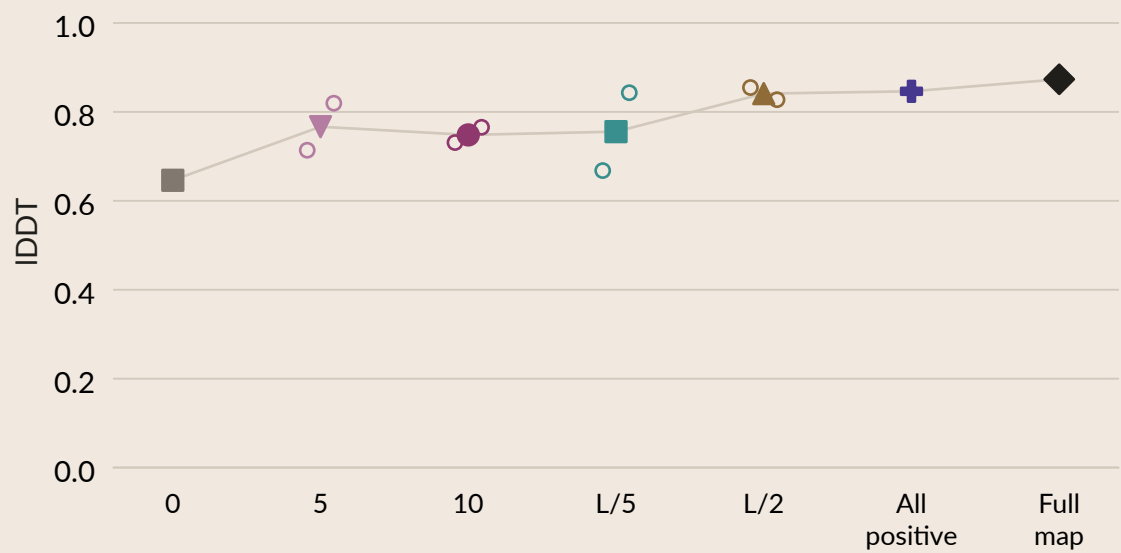
8wrx_A • depth 4 • L = 88
