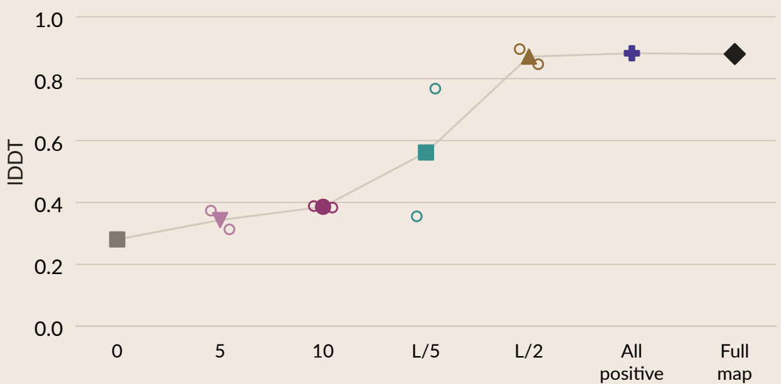
8oxk_A • depth 6 • L = 99
