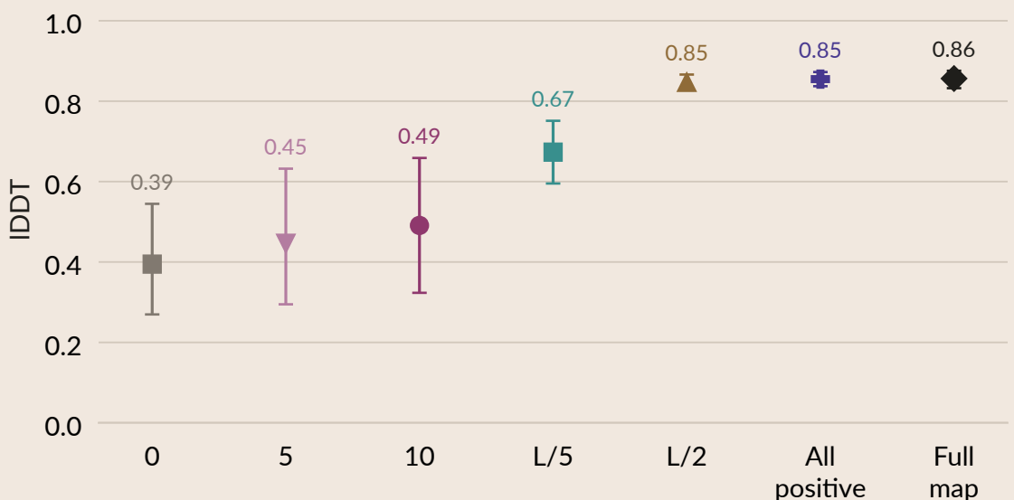
Mean of five proteins • 95% protein interval
