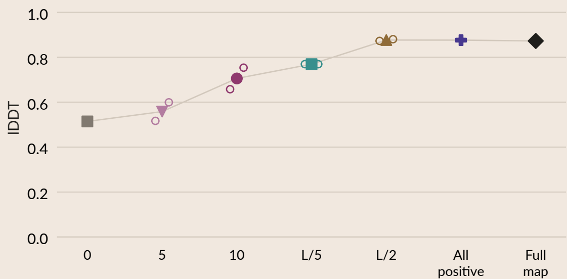
8ii8_A • depth 3 • L = 226
