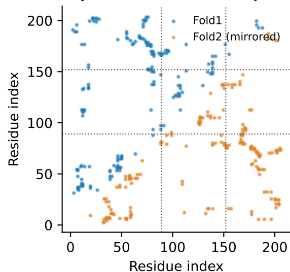
Experimental contact maps
