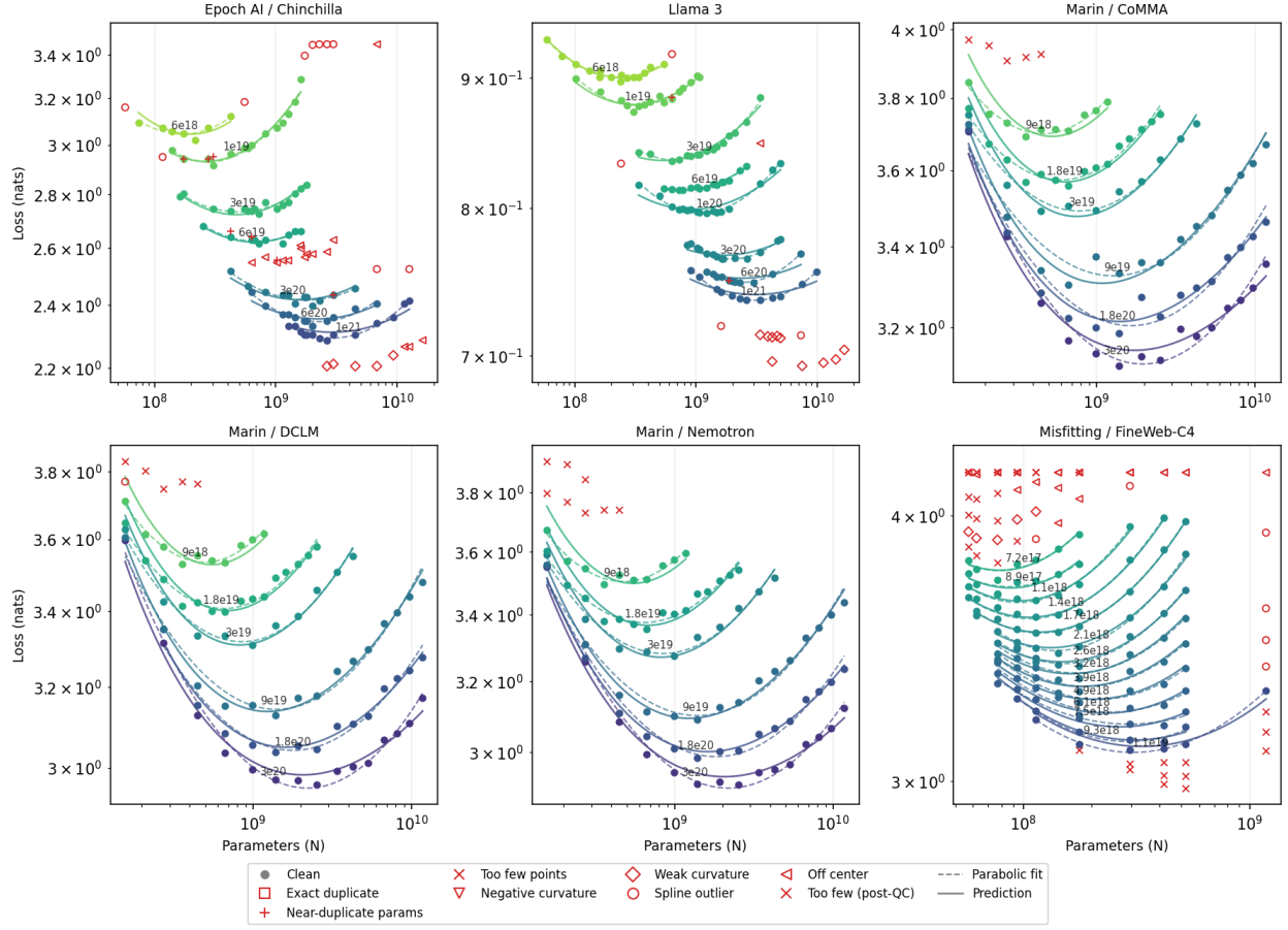
Figure A1: IsoFLOP curves for six experiments spanning different datasets and model families. Clean points (circles) and outlier points (markers by reason) are shown alongside parabolic fits (dashed) and Approach 3 predictions with per-budget FLOP factor adjustment (solid). Experiments shown: Epoch AI/Chinchilla, Llama 3, Marin/CoMMA, Marin/DCLM, Marin/Nemotron, and Misfitting/FineWeb-C4.
