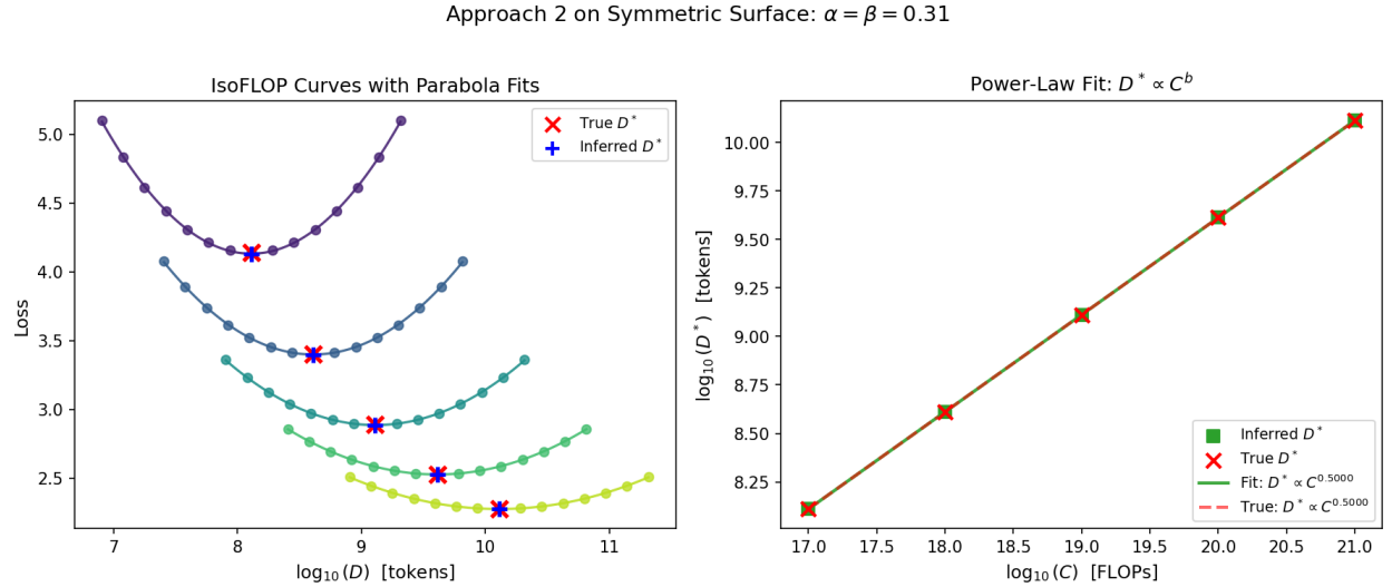
Figure 3: Approach 2 applied to a symmetric loss surface. Left: IsoFLOP curves with fitted parabolas. True ( \times ) and inferred ( + ) optima are indistinguishable. Right: Power-law fit recovers the exact scaling exponent.
