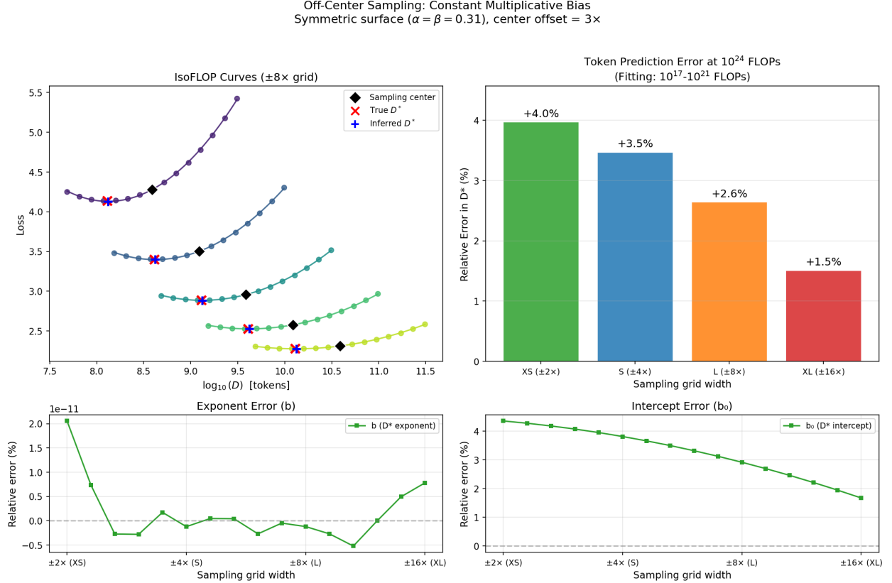
Figure 6: Effect of a constant 3\times offset in sampling centers on the symmetric surface. Top left: IsoFLOP curves at the Large grid ( \pm 8\times ), with black diamonds marking the (off-center) sampling center, red \times the true D^* , and blue + the inferred D^* . Top right: extrapolation error in compute-optimal token prediction at 10^{24} FLOPs for each grid width. Bottom row: exponent and intercept errors across grid widths from XS ( \pm 2\times ) to XL ( \pm 16\times ), plotted on the same y-axis scale. The exponent is recovered perfectly (flat at zero) while the intercept shows systematic bias that varies with grid width.
