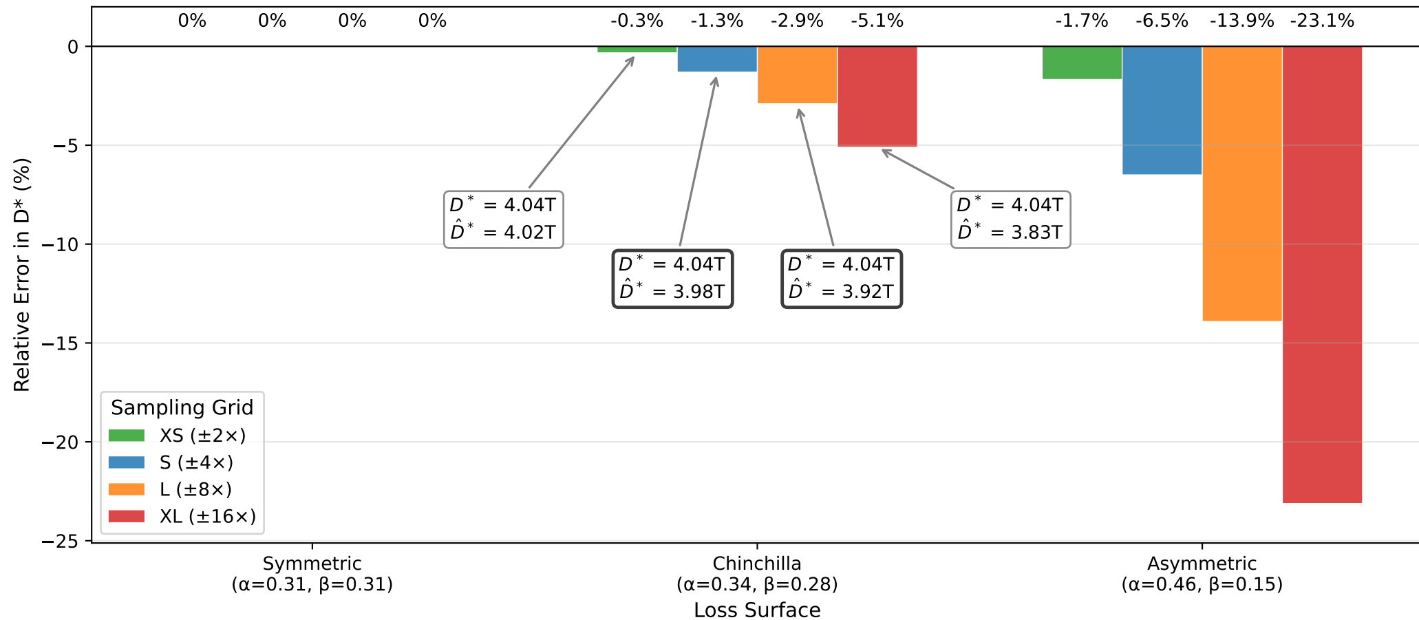
Token Prediction Error by Surface and Grid Width (Fitting: 10^{17} - 10^{21} FLOPs → Extrapolating to 10^{24} FLOPs)
