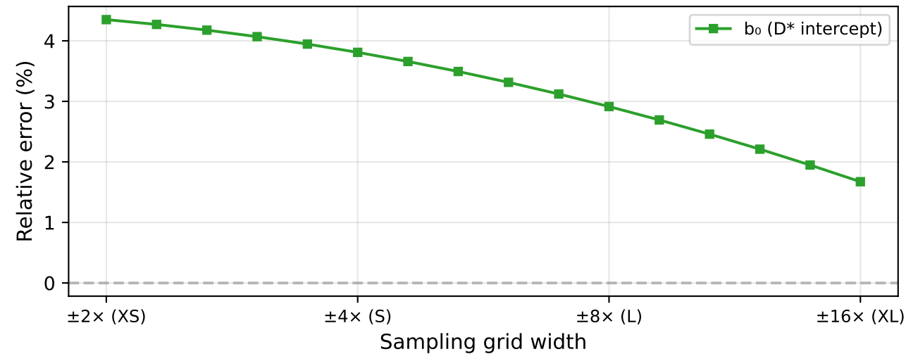
Intercept Error ( b_0 )
