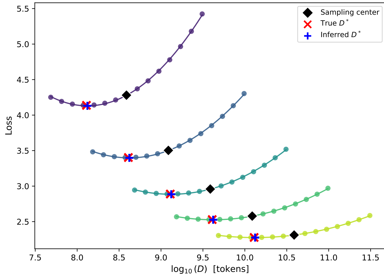
IsoFLOP Curves ( \pm 8\times grid)
