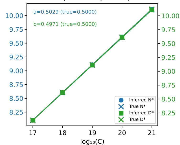
N^*, D^* vs C ( \pm 100x )
