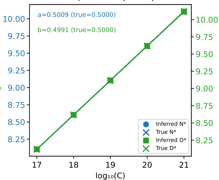
N^*, D^* vs C ( \pm 16x )
