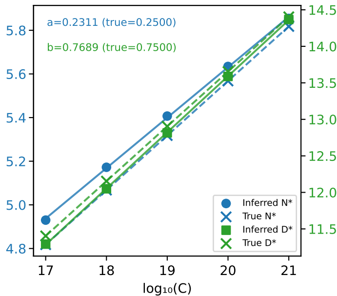
N^* , D^* vs C ( \pm 16x )
