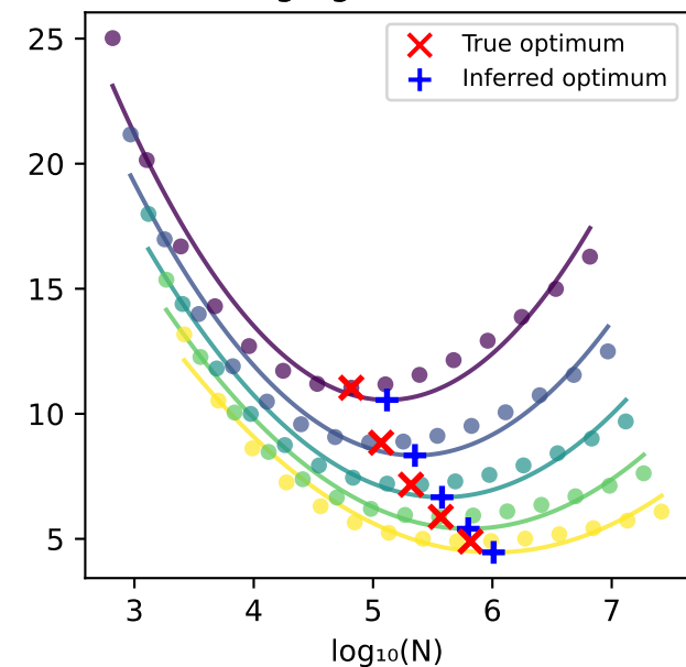
Large grid ( \pm 100x )
