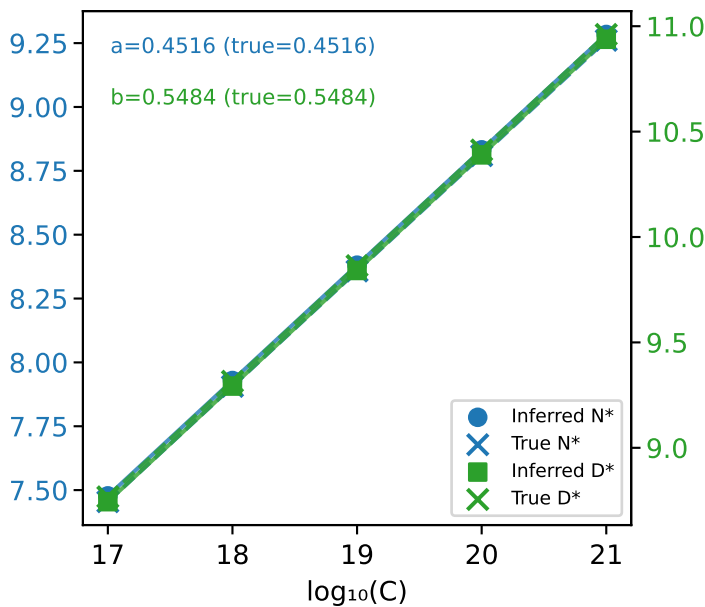
N^* , D^* vs C ( \pm 16x )
