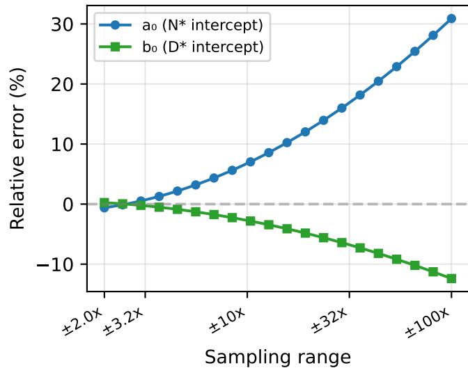
Intercept Error
