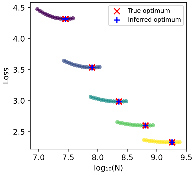
Small grid ( \pm 2.0x )
