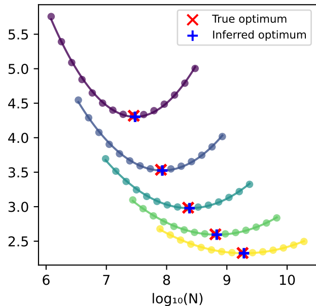
Medium grid ( \pm 16x )
