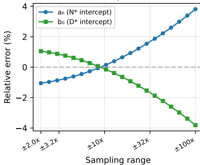
Intercept Error
