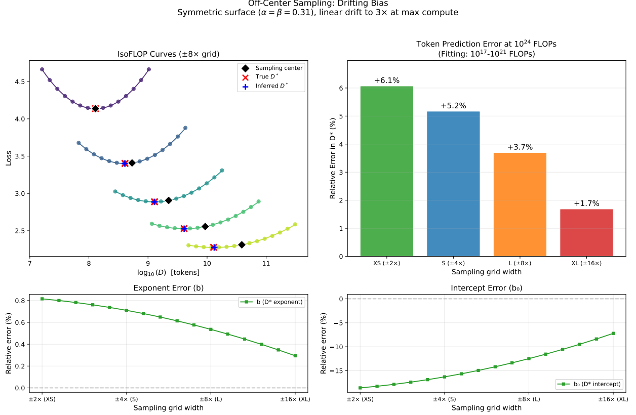
Figure 7: Effect of a linear drift in sampling centers (centered at true optimum for lowest budget, drifting to 3\times at highest budget) on the symmetric surface. Unlike the constant bias case, the exponent error (bottom left) is now non-zero: the slope of \log D^* vs \log C is distorted because the offset varies across compute budgets.
