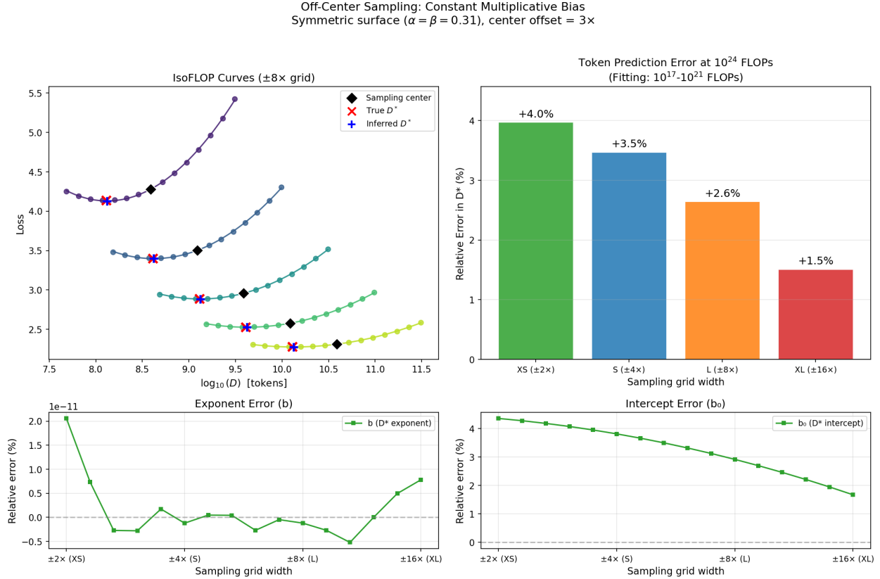
Figure 6: Effect of a constant 3\times offset in sampling centers on the symmetric surface. Top left: IsoFLOP curves at the Large grid ( \pm 8\times ), with black diamonds marking the (off-center) sampling center, red \times the true D^* , and blue + the inferred D^* . Top right: extrapolation error in compute-optimal token prediction at 10^{24} FLOPs for each grid width. Bottom row: exponent and intercept errors across grid widths from XS ( \pm 2\times ) to XL ( \pm 16\times ), plotted on the same y-axis scale. The exponent is recovered perfectly (flat at zero) while the intercept shows systematic bias that varies with grid width.
