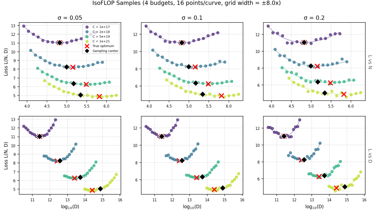
Figure 15: Noisy IsoFLOP samples used in the exponent inference comparison (Figure 9). Columns correspond to noise levels ( \sigma = 0.05, 0.1, 0.2 ); rows show loss versus \log_{10}(N) (top) and \log_{10}(D) (bottom). Scatter points are noisy observations; solid curves show the noiseless reference surface. Red \times marks the true compute-optimal point at each budget; black diamonds mark the sampling centers, which drift away from the true optima at higher compute budgets. Surface: Asymmetric ( \alpha = 0.465, \beta = 0.155 ), 4 budgets ( 10^{17} – 10^{21} FLOPs), 32 points per curve, \pm 8\times grid.
