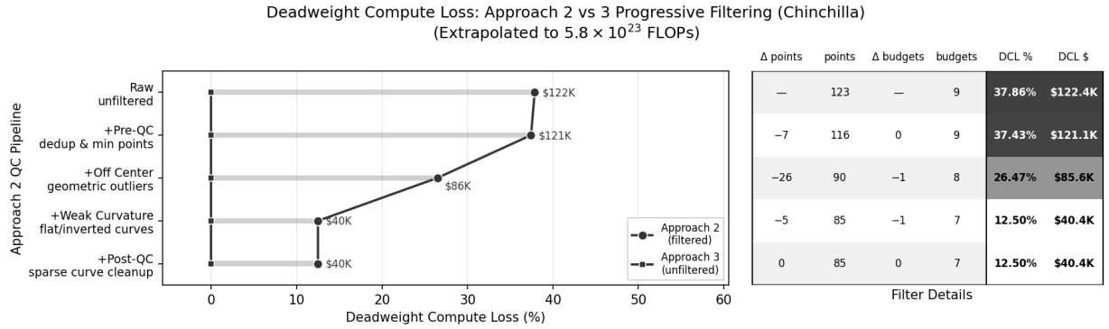
Figure 19: Progressive quality control filtering on Chinchilla data, analogous to Figure 12 for Llama 3. DCL is measured against an Approach 3 surface fit to unfiltered data and extrapolated to 5.8 \times 10^{23} FLOPs. Starting from 37.9% DCL on raw data, the off-center and weak-curvature filters reduce DCL to 12.5%.
