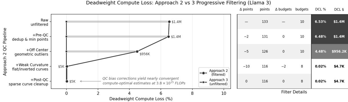
Figure 12: Effect of progressive quality control filtering on Approach 2 Deadweight Compute Loss, measured against an Approach 3 surface fit to unfiltered Llama 3 data. Each row cumulatively applies one QC stage. Nearly all DCL reduction comes from the off-center and weak-curvature filters, which target the specific Approach 2 biases identified in this study. The right table reports points and budgets removed at each stage, along with DCL as a percentage of the 3.8 \times 10^{25} FLOP evaluation budget and dollar cost.
