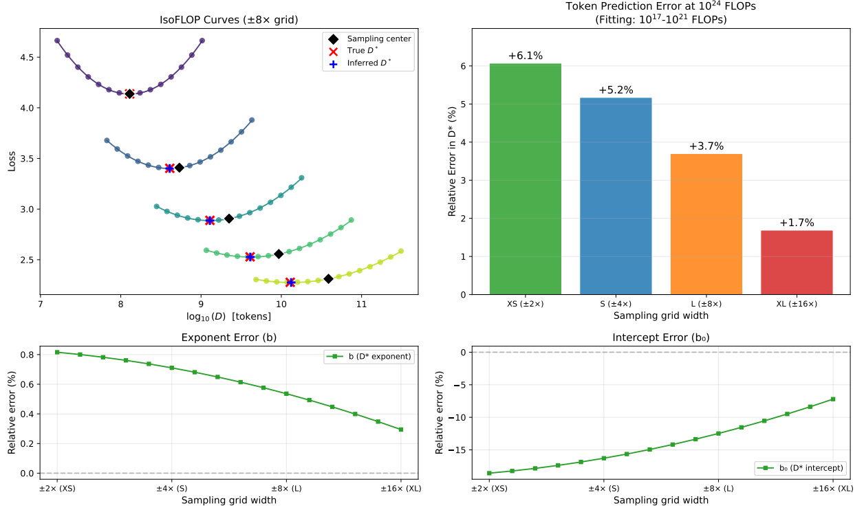
Figure 7: Effect of a linear drift in sampling centers (centered at true optimum for lowest budget, drifting to 3\times at highest budget) on the symmetric surface. Unlike the constant bias case, the exponent error (bottom left) is now non-zero: the slope of \log D^* vs \log C is distorted because the offset varies across compute budgets.
