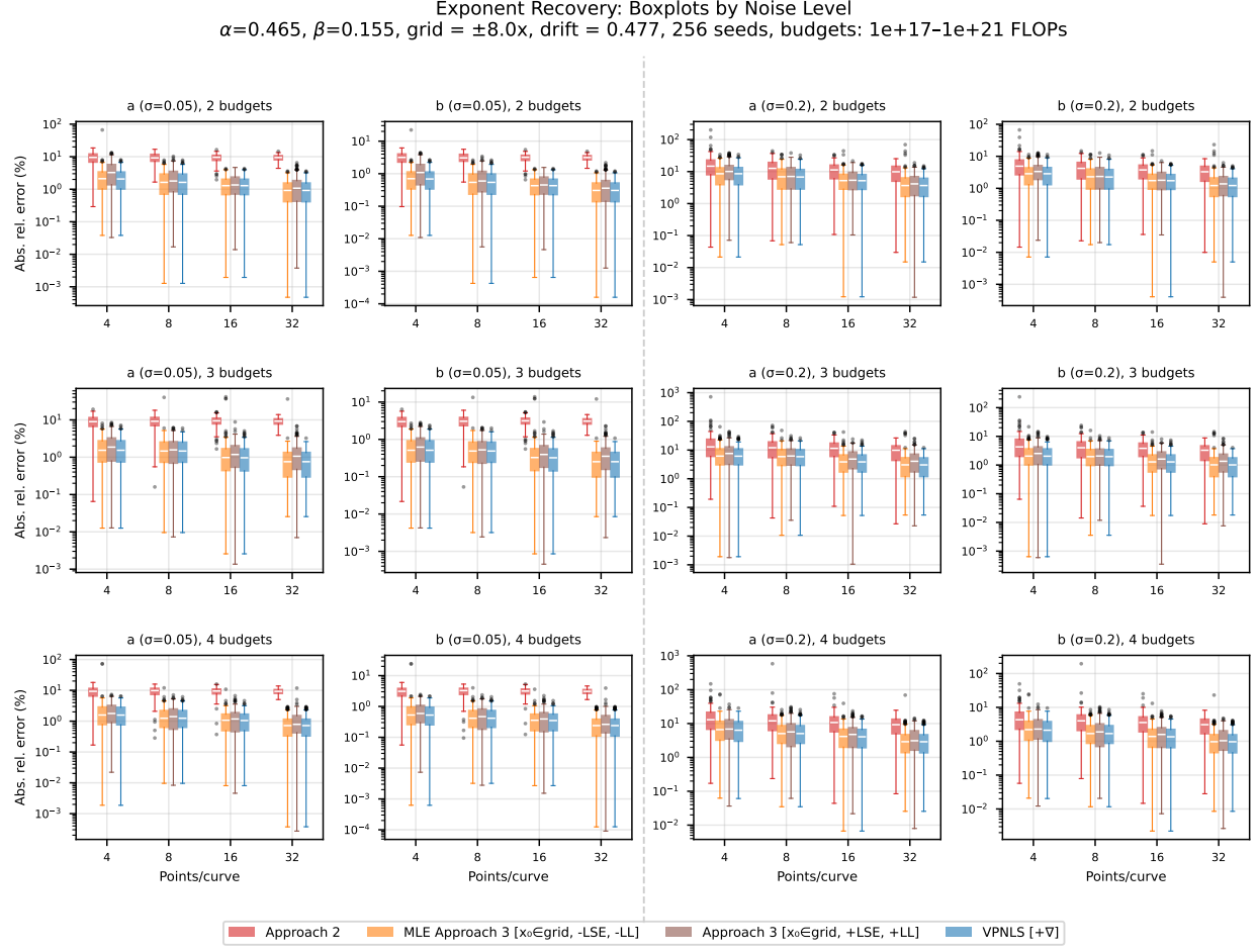
Figure A5: Per-condition breakdown of exponent inference errors from Figure 11, showing 4 of 5 methods (excludes Naive Approach 3, which serves only as a negative control in the main figure). Rows correspond to number of compute budgets (2, 3, 4); left columns show the lowest noise level ( \sigma = 0.05 ) and right columns show the highest ( \sigma = 0.2 ), each split by exponent ( a and b ). Within each panel, boxplots show absolute relative error (%) on a log scale for each method at each points-per-curve setting (4, 8, 16, 32), over 256 noise realizations.
