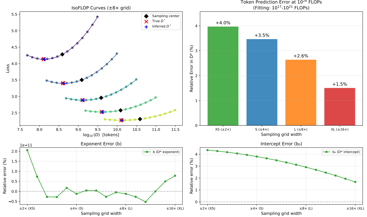
Figure 6: Effect of a constant 3\times offset in sampling centers on the symmetric surface. Top left: IsoFLOP curves at the Large grid ( \pm 8\times ), with black diamonds marking the (off-center) sampling center, red \times the true D^* , and blue + the inferred D^* . Top right: extrapolation error in compute-optimal token prediction at 10^{24} FLOPs for each grid width. Bottom row: exponent and intercept errors across grid widths from XS ( \pm 2\times ) to XL ( \pm 16\times ), plotted on the same y-axis scale. The exponent is recovered perfectly (flat at zero) while the intercept shows systematic bias that varies with grid width.
