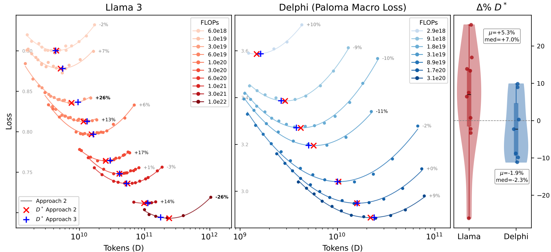
Figure 3: IsoFLOP curves with Approach 2 parabolic fits ( L vs \log D ) and inferred D^* vertices from Approach 2 (x) and Approach 3 (+).
