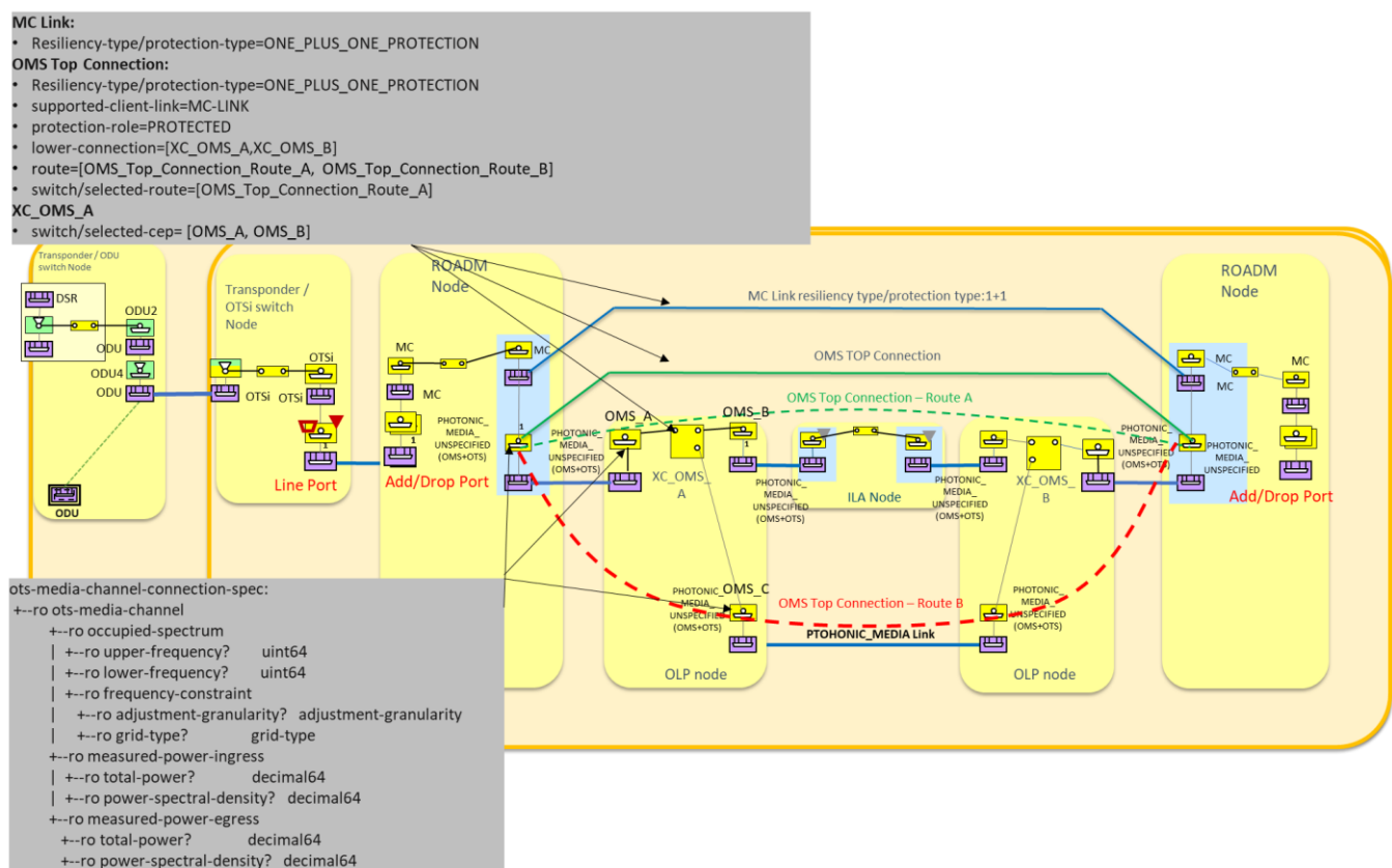
Figure 6-36 UC-5a OLP protection TAPI representation. Note that Route A and Route B represented as dashed lines are not connections (only refer to routes of the single OMS top connection).
