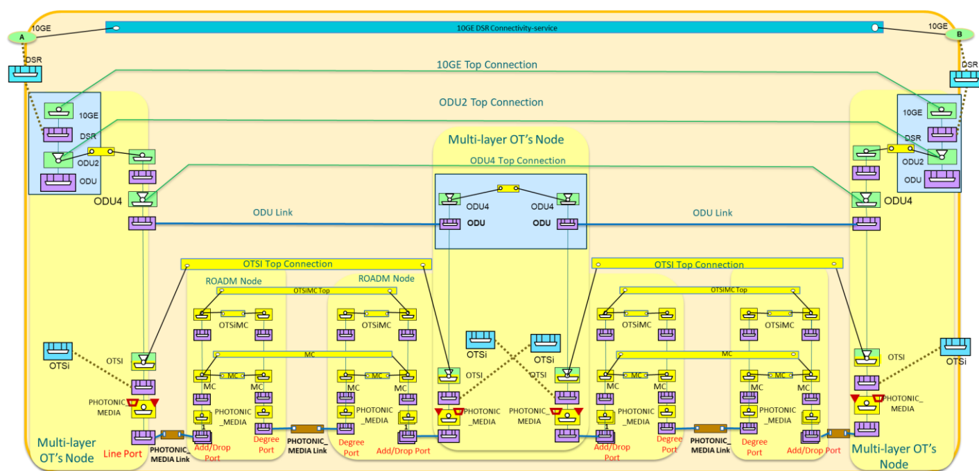
Figure 6-17 Connectivity Service 10GE client signal over ODU2 over ODU4 (Fixed DSR-ODU mapping, flexible ODU allocation) with intermediate transponder regeneration.
