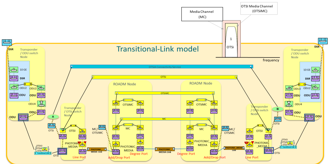
Figure 6-25 OTSi single lambda connectivity-service - Transitional link model.
