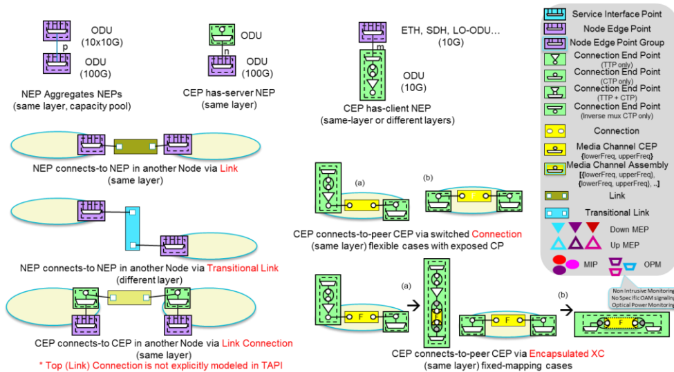
Figure 6-11 TAPI Logical Termination Point Template – Basic Arrangements.
