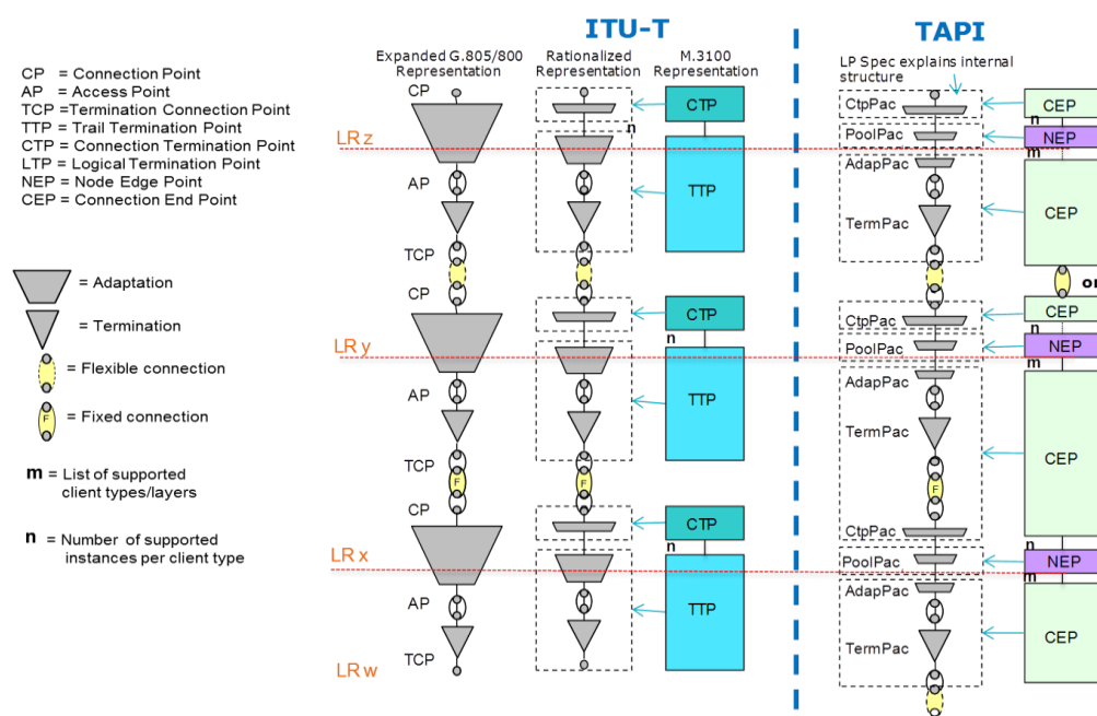
Figure 3-2 TAPI Mapping from ITU-T.
