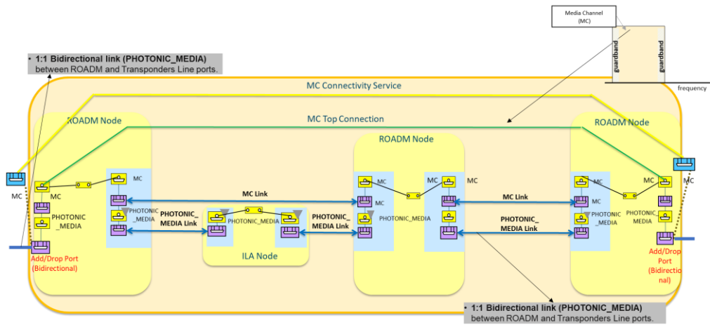
Figure 6-29 Full Bidirectional - UNI and OMS bidirectional scenario.
