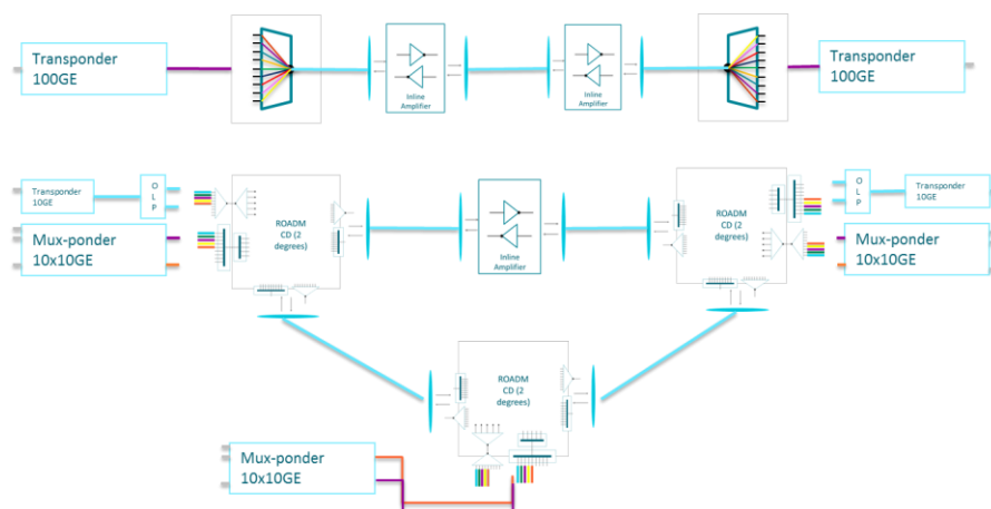
Figure 4-7 NS-2: OTN/WDM Network scenario 2.
