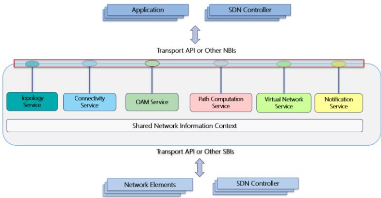
Figure 3-1 Transport API Functional Architecture
