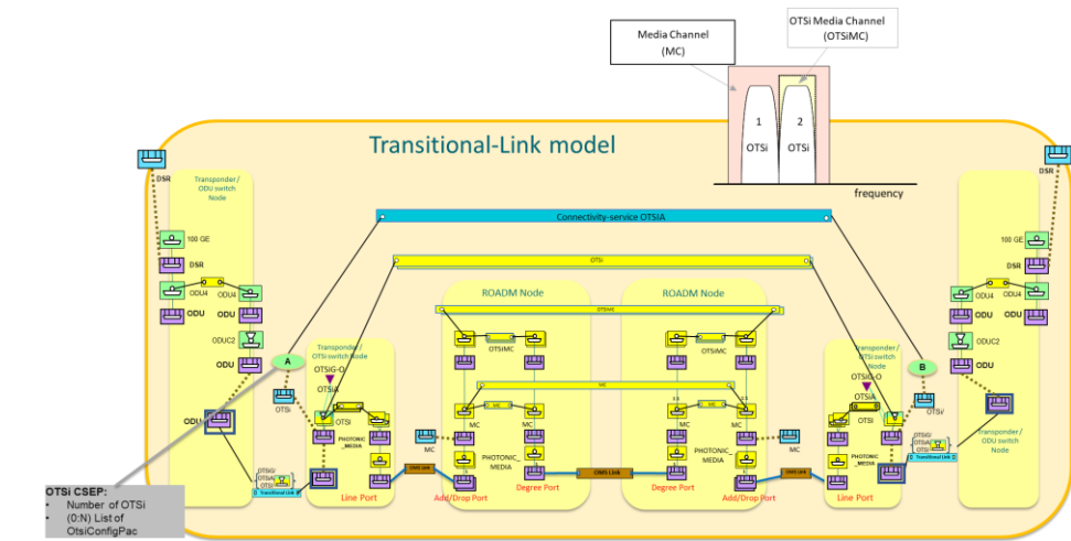
Figure 6-27 OTSiA multi-wavelength connectivity-service (transitional link model abstraction).
