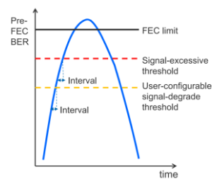
Figure 3-6 FEC function related thresholds
