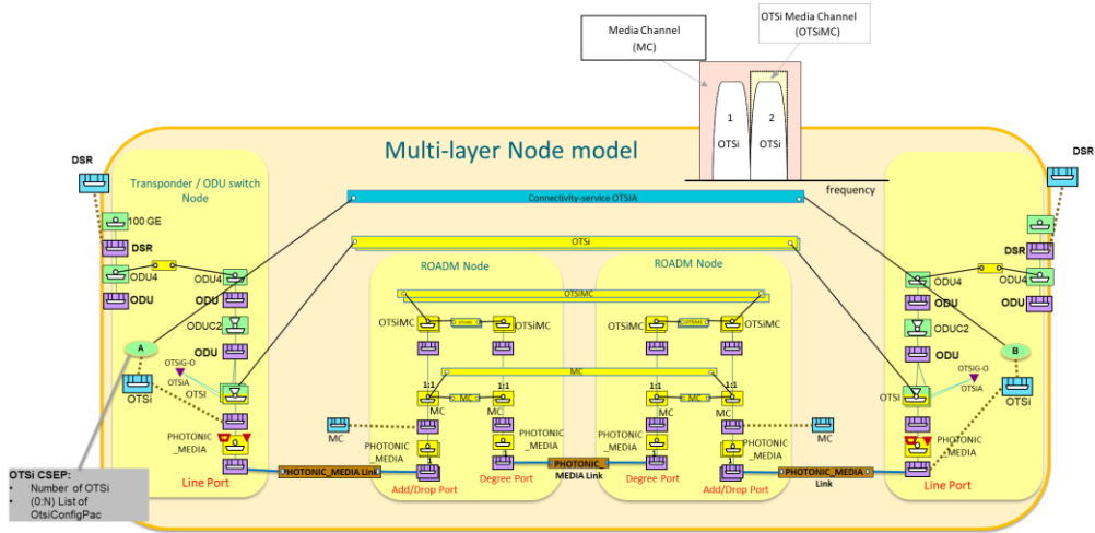
Figure 6-28 OTSiA multi-wavelength connectivity-service (multi-layer node model abstraction).
