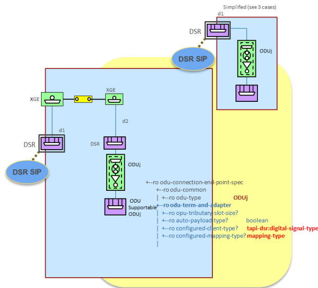
Figure 6-20 UC-1c Client port representation - initial state.
