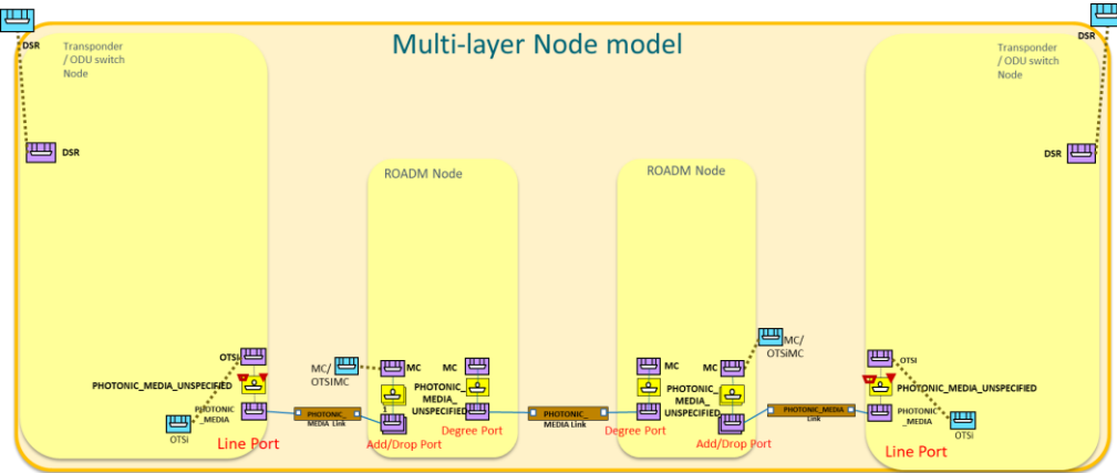
Figure 6-4 TAPI topology representation at "day 0" following Multi-layer Node modelling approach. 6.1.3 Use case 0c: Connectivity Service and Connection discovery (synchronous mode) Number UC0c Name Connectivity Service and Connection discovery (synchronous mode)
