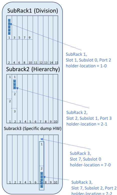
Figure 6-35 UC-4b Network Element Subracks container-holder location examples.
