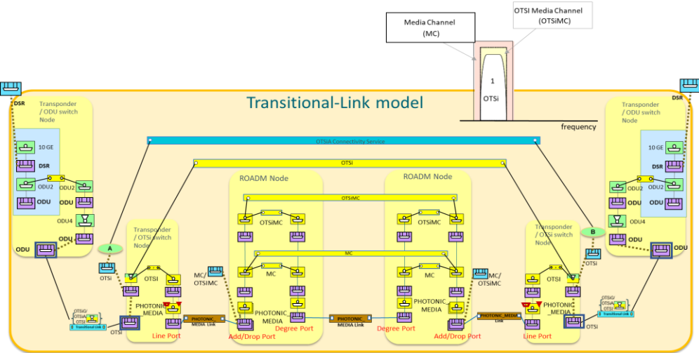
Figure 6-25 OTSi single lambda connectivity-service - Transitional link model.
