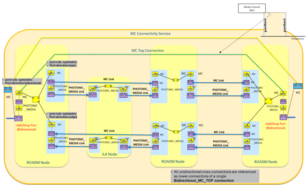
Figure 6-30 Mixed Scenario - UNI bidirectional and OMS unidirectional.
