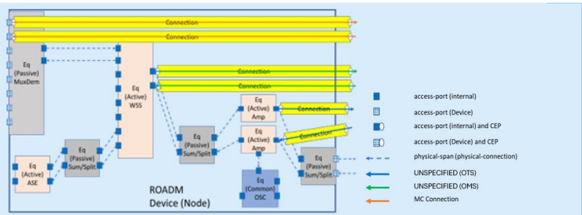
Figure 6-6: TOP Connection and Equipment within a ROADM Device
