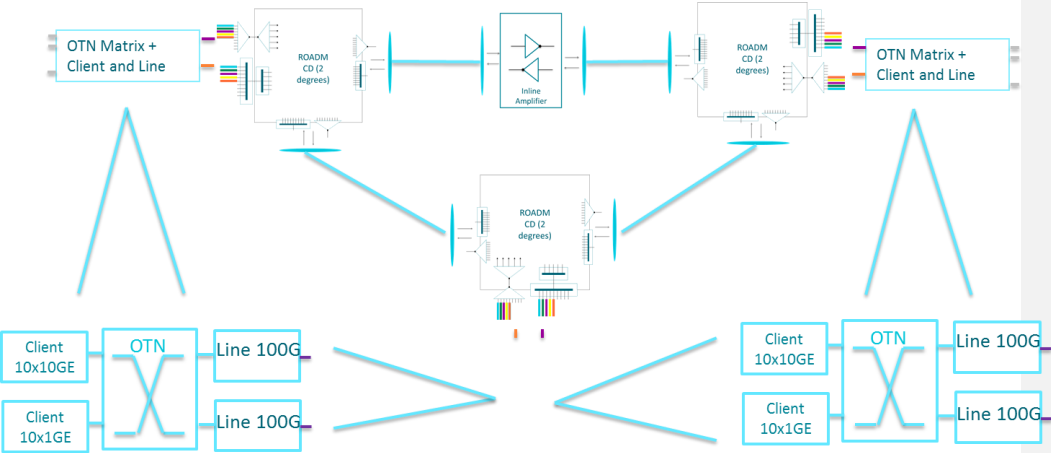
Figure 4-2 NS-1: OTN/WDM Network scenario
