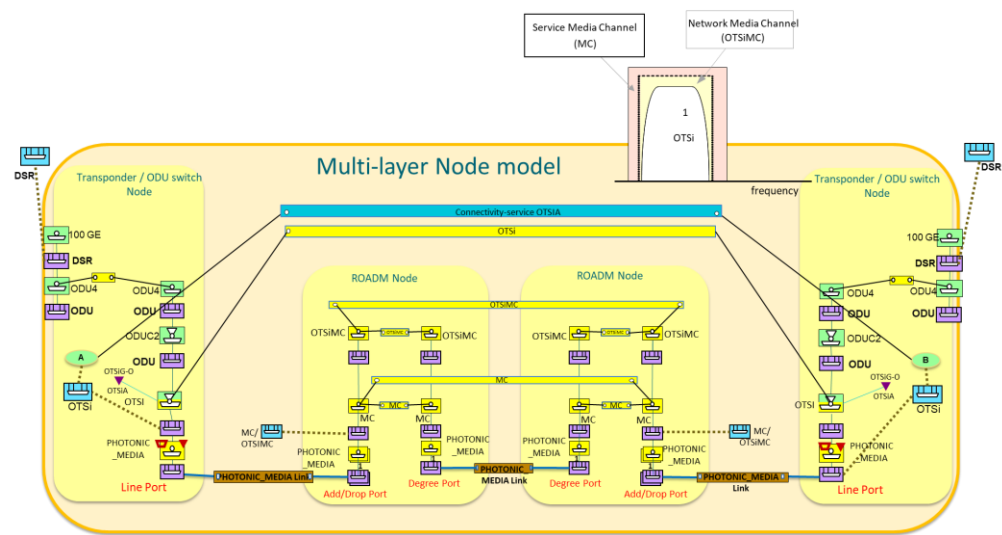
Figure 6-26 OTSi single lambda connectivity-service - Multi-layer node approach.
