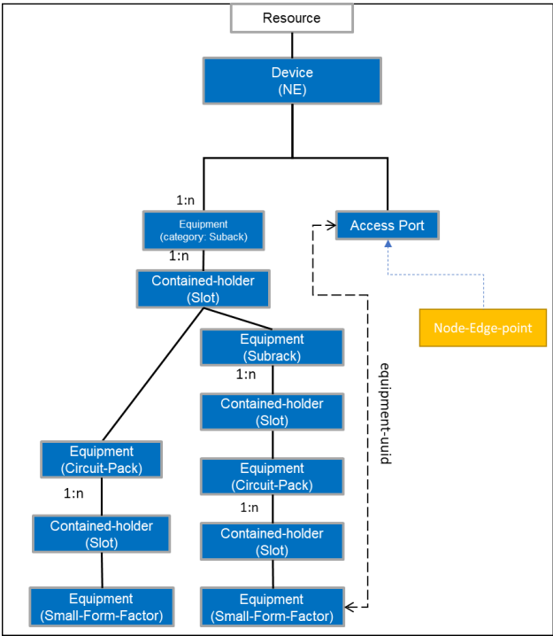
Figure 6-34 UC-4b Hierarchical arrangement of equipment objects.
