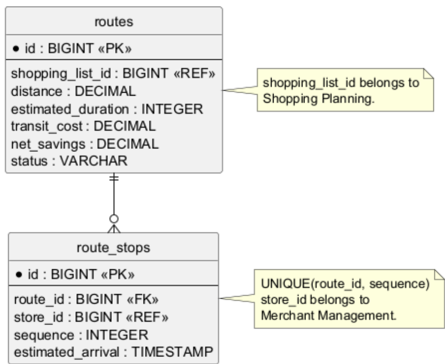
Preciazo - Route Planning Database Diagram
