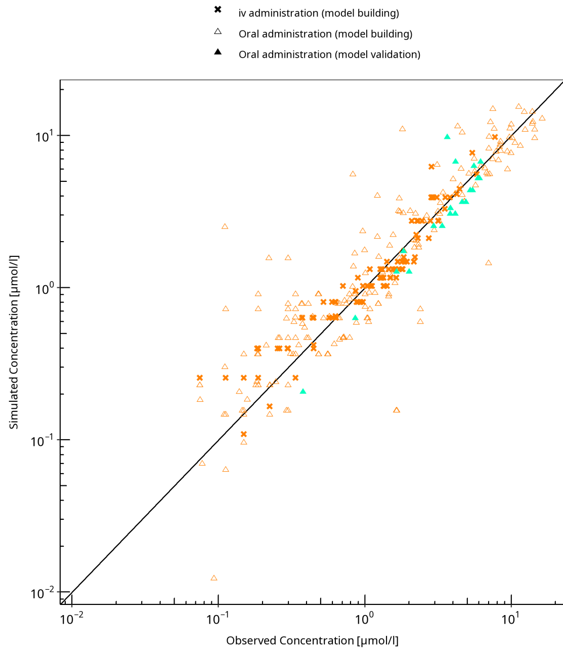
Figure 3-1: Moclobemide concentration in plasma
