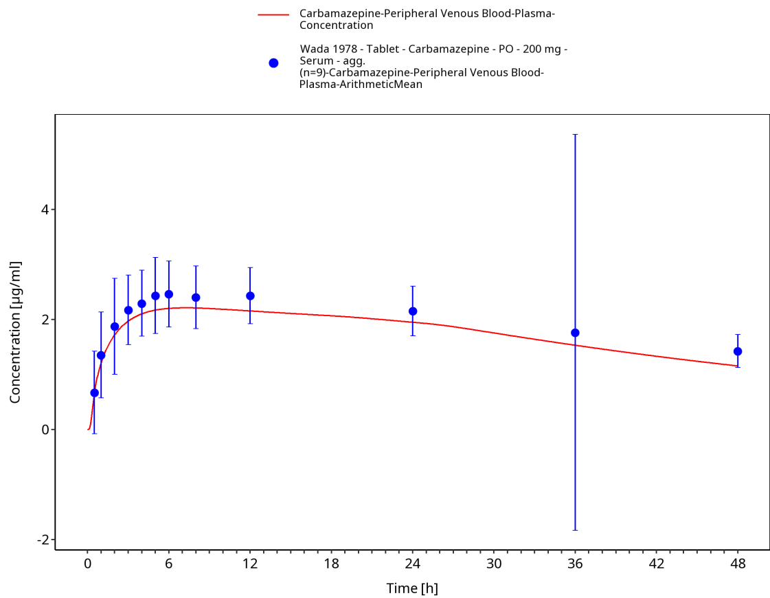
Figure 3-62: Wada1978_200mg_sd_tablR_plasma
