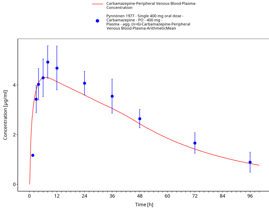
Figure 3-41: Pynnoenen1977_400mg_sd_tabIR_plasma
