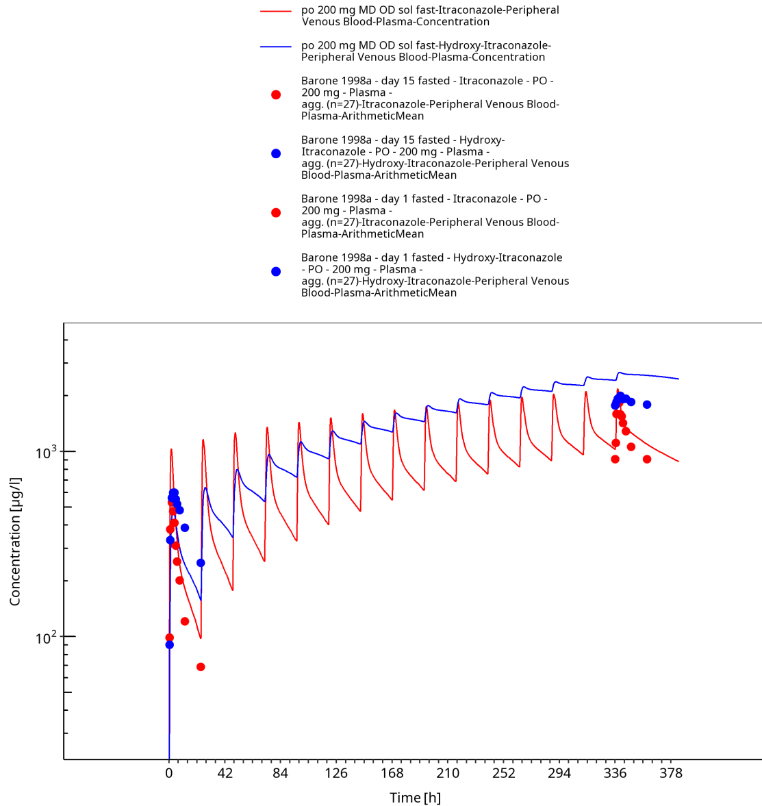
Figure 3-25: po 200 mg MD OD sol fast - Plasma
