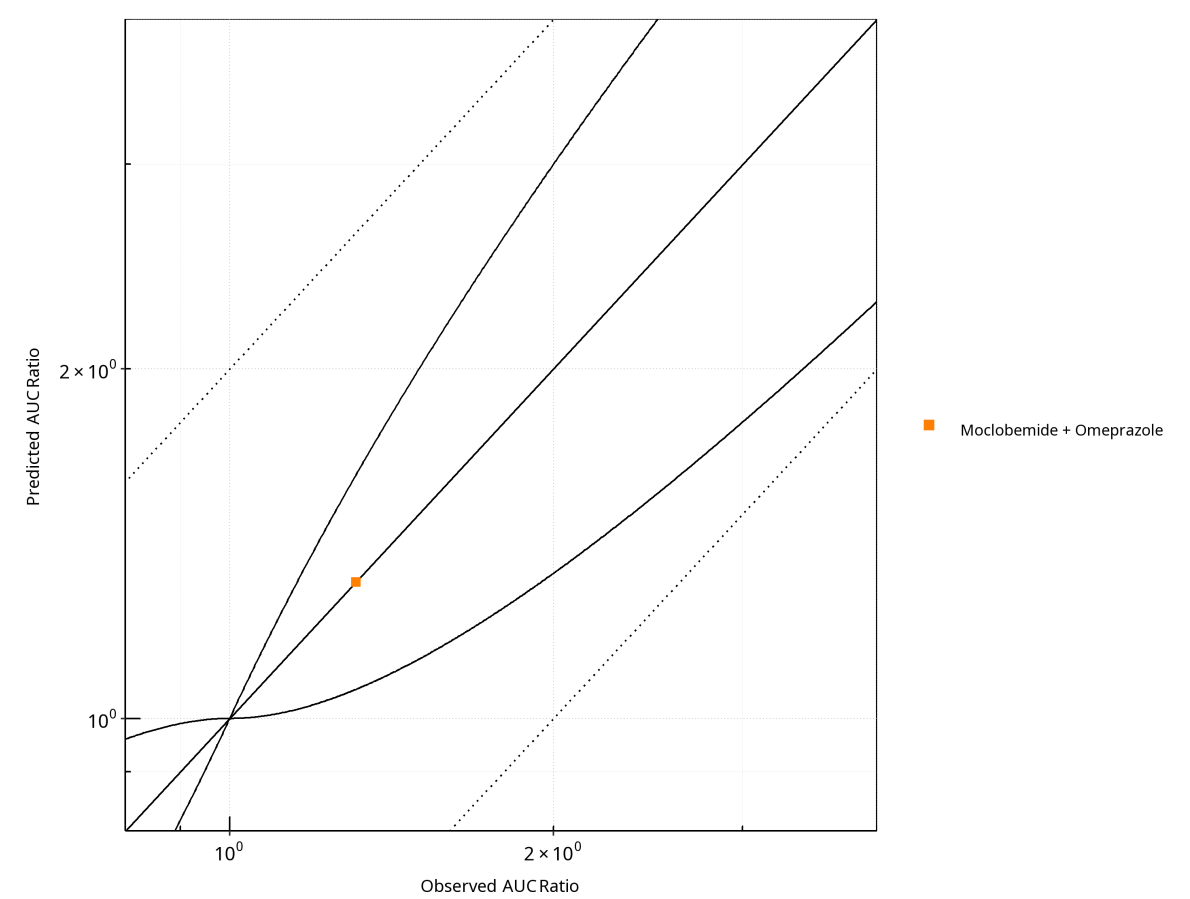
Figure 2-17: CYP2C19 DDI. Victim: Moclobemide . Predicted vs. Observed AUC Ratio. ( \delta = 1 in Guest et al. formula)
