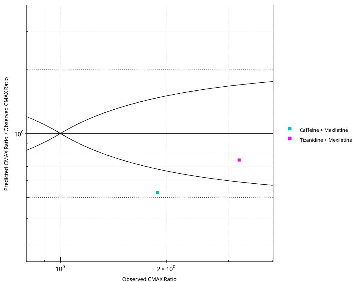
Figure 2-16: CYP1A2 DDI. Perpetrator: Mexiletine. Predicted/Observed vs. Observed CMAX Ratio. ( \delta = 1 in Guest et al. formula)
