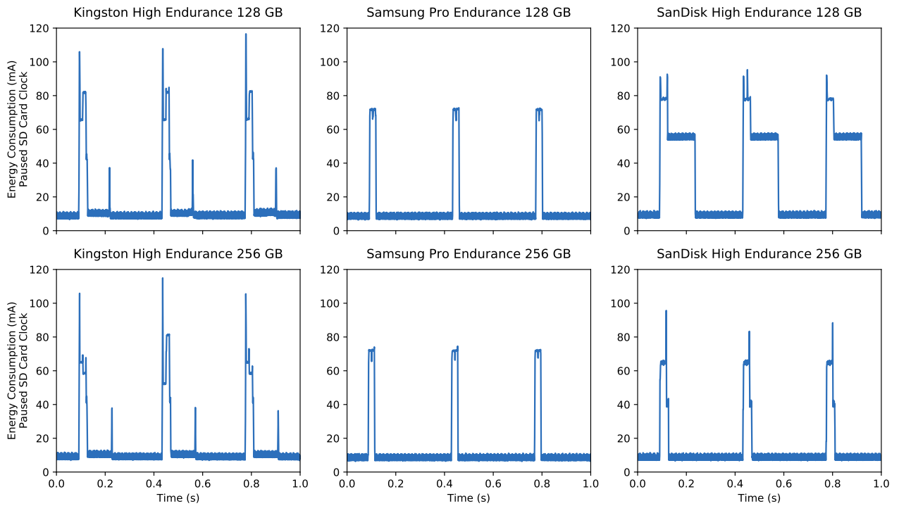
Figure 4: Energy consumption of AudioMoth using multiple SD cards when recording at 48 kHz using the updated version of the AudioMoth firmware which pauses the SD clock between writes.
