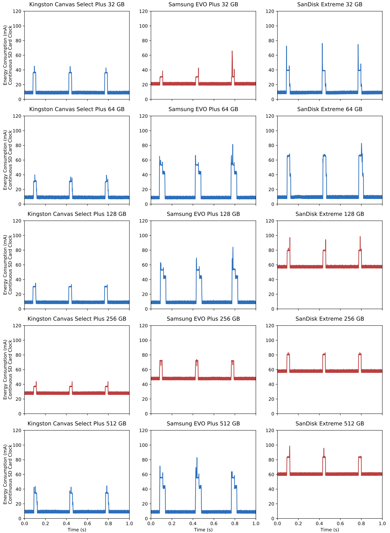
Figure 1: Energy consumption of AudioMoth using multiple SD cards when recording at 48 kHz using the previous versions of the AudioMoth firmware which do not pause the SD clock between writes.
