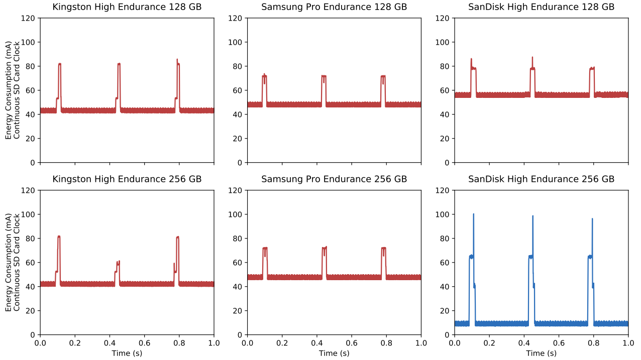
Figure 3: Energy consumption of AudioMoth using multiple SD cards when recording at 48 kHz using the previous versions of the AudioMoth firmware which do not pause the SD clock between writes.
