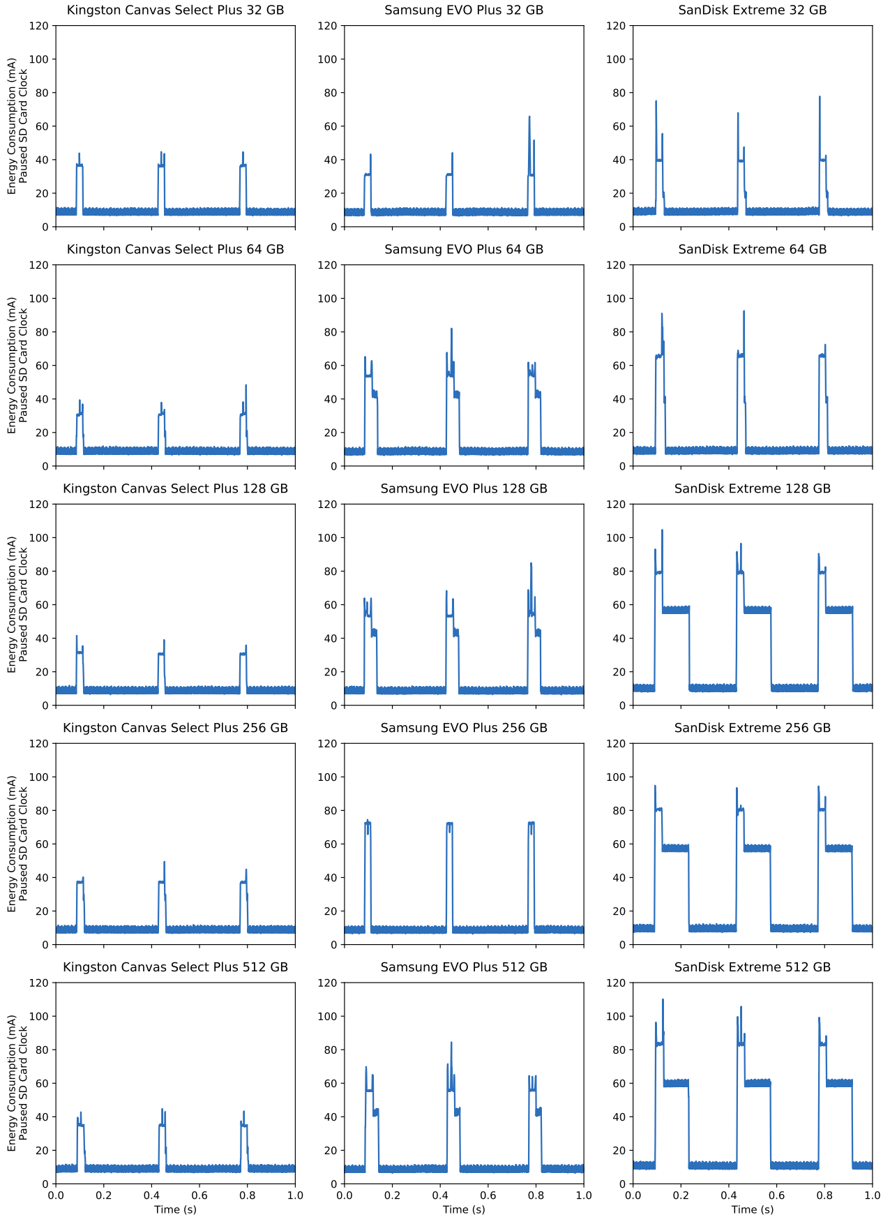
Figure 2: Energy consumption of AudioMoth using multiple SD cards when recording at 48 kHz using the updated version of the AudioMoth firmware which pauses the SD clock between writes.
