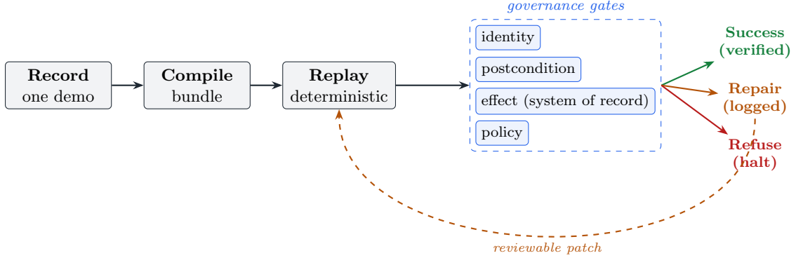
Figure 1: OpenAdapt compiles one demonstration into a deterministic program. Healthy replay makes no model calls. Each step passes governance gates; the runtime verifies and succeeds, records a bounded repair when a lower-fidelity rung re-resolves a changed target, or refuses when a configured check cannot be verified. A repair is an auditable patch, never a silent overwrite of the deployed bundle.
