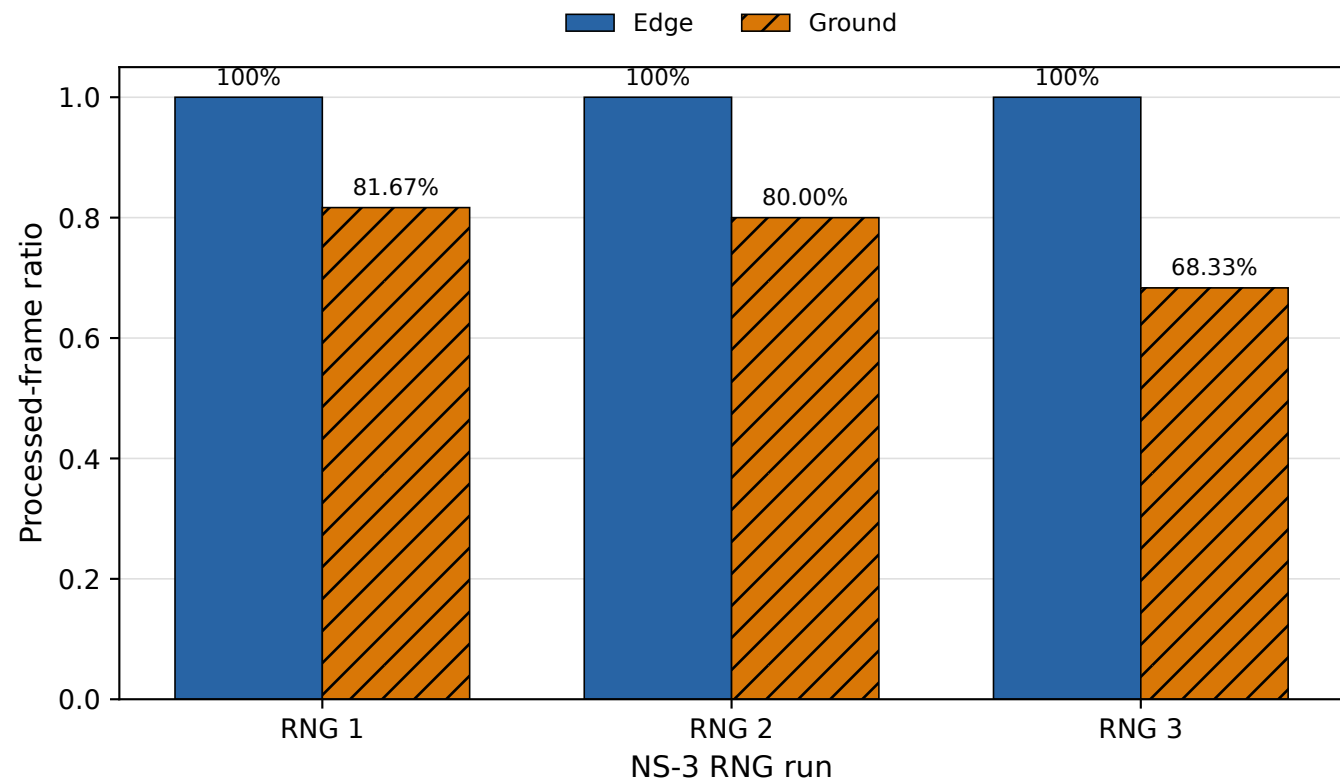
Processed-Frame Completion by RNG Run Edge: local pipeline; Ground: complete compressed-frame processing
