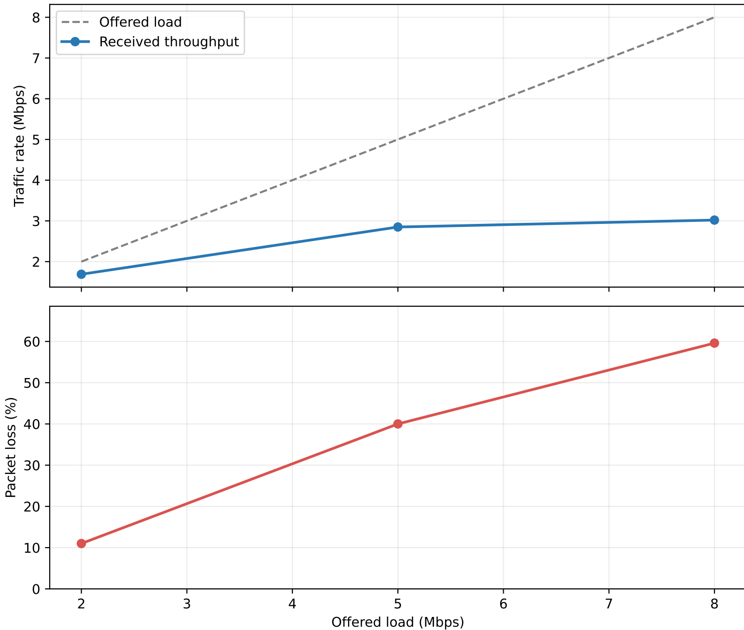
Throughput and Loss Against Offered Load
