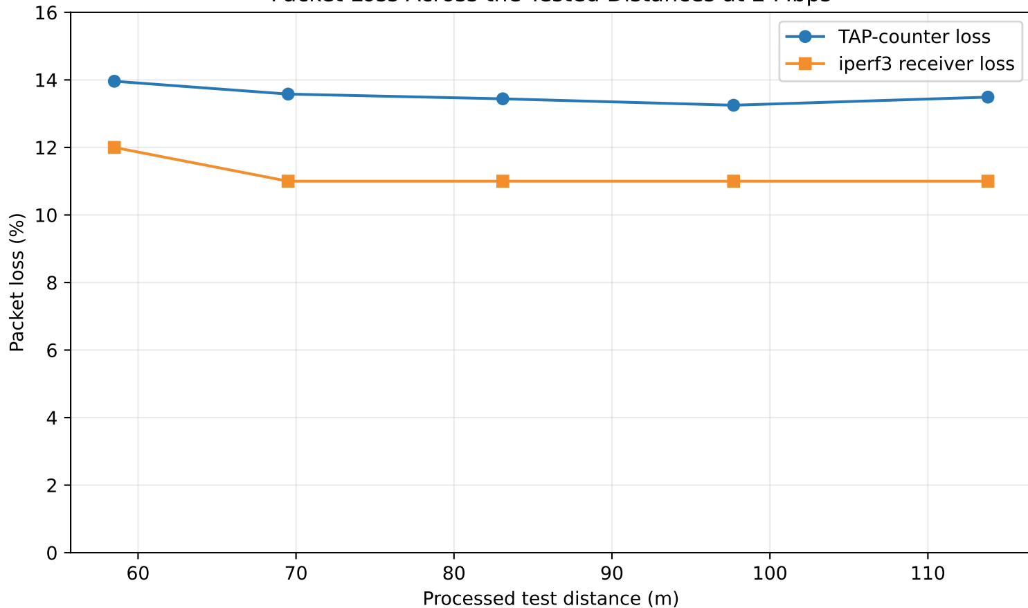
Packet Loss Across the Tested Distances at 2 Mbps
