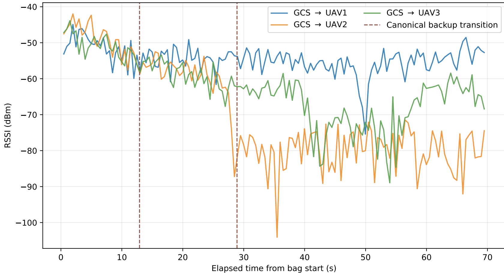
Corrected Trial 1 GCS-to-UAV RSSI
