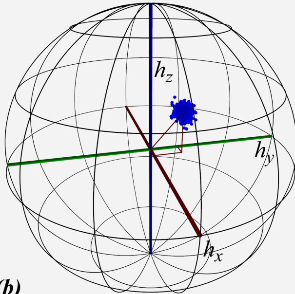
Homochoric
